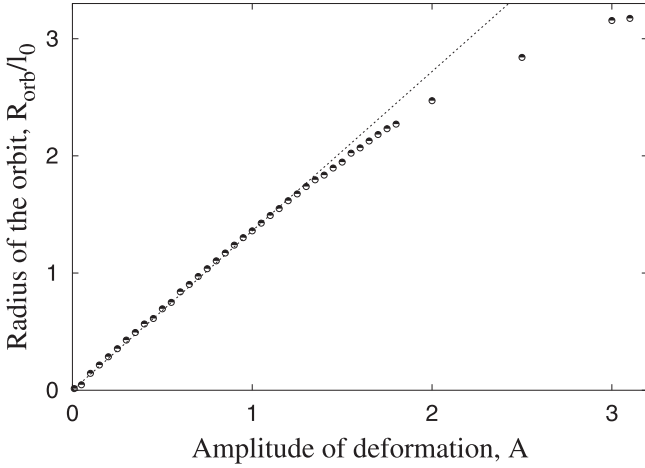
Fig. 6. Radius of the soliton orbit as a function of the deformation amplitude A . Parameters of the soliton: initial radius R = 4.87l_0 and initial precession frequency \omega_p = 0.2\omega_0 .
