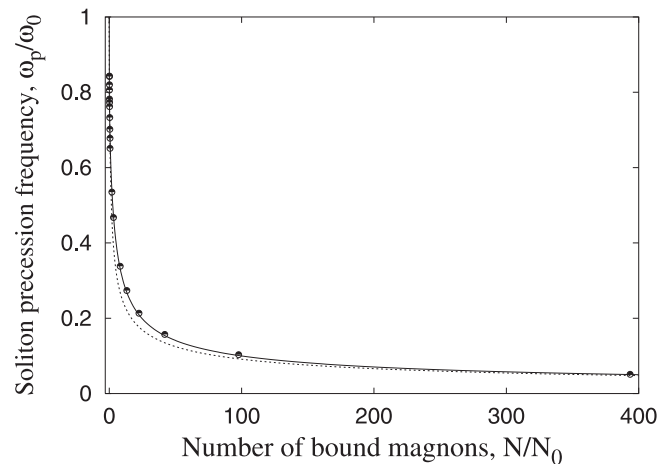
Fig. 2. Soliton precession frequency as a function of the number of bound magnons. Symbols correspond to the simulation data; the solid line is the result of continuum model integration; the dashed line corresponds to equation (32).
