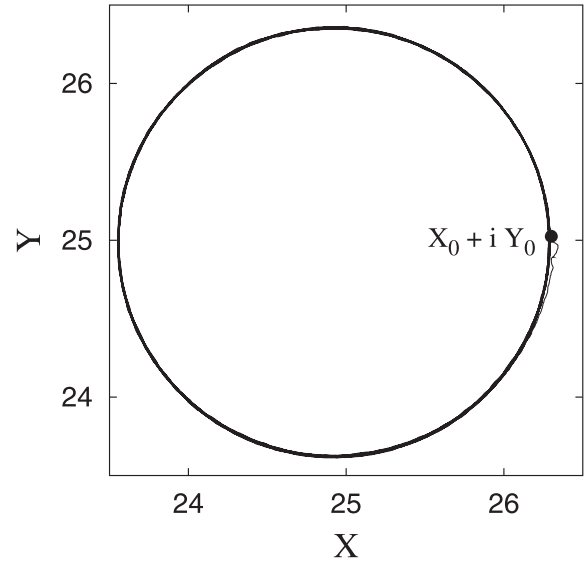
Fig. 4. Trajectory of the soliton with initial radius R = 4.87l_0 and initial precession frequency \omega_p = 0.2\omega_0 . The initial point X_0 + iY_0 corresponds to the center of the soliton from Figure 3.
