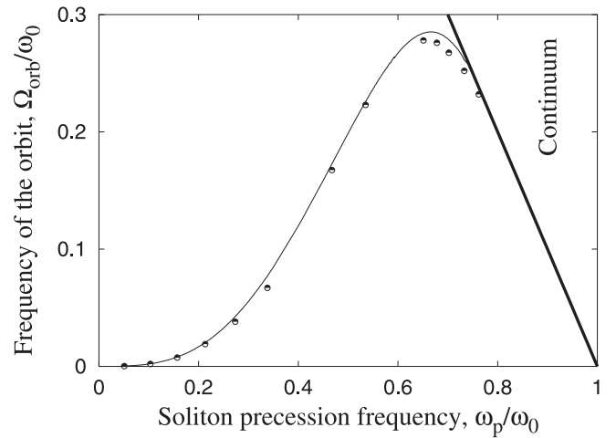
Fig. 5. Frequency of the orbit motion as a function of the precession frequency of the soliton. Symbols correspond to the spin dynamics simulation data; lines corresponds to the frequency of the eigenmode with m = -1 from the continuum theory by Sheka et al. [20].
