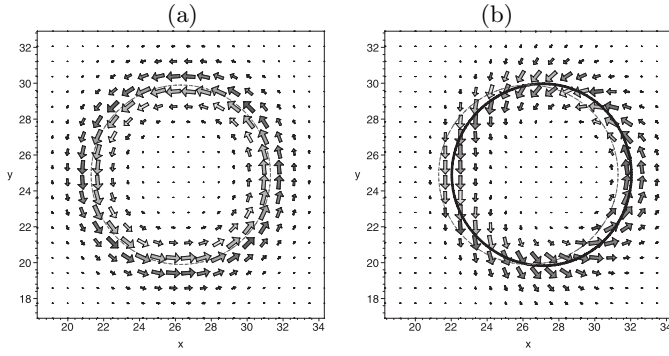
Fig. 3. In-plane spin distribution for the soliton with R = 5l_0 , which is situated at \mathbf{X}_0 = 26.3 + i25.0 . (a) corresponds to the circular symmetric soliton and (b) to an elliptically deformed one. The lines describe the contour plot of S_z = 0 ( \theta = \pi/2 ): the dashed line is for the circular symmetric soliton and the solid line is for the deformed soliton.
