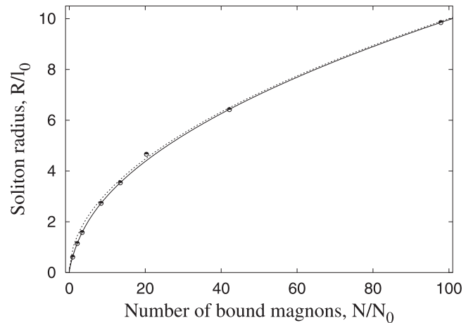
Fig. 1. Soliton radius as a function of the number of bound magnons. The symbols correspond to the simulation data; the solid line is the result of the numerical integration of the continuum limit equations (11), (12) using the one-parameter shooting method with the 4th-order Runge-Kutta scheme. The dashed line corresponds to equation (31).
